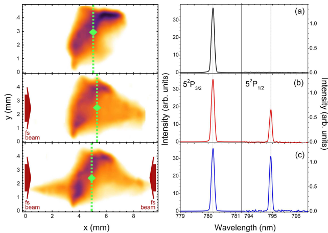
FIG. 5. (Color online) Fluorescence intensity distribution (left panel) and LIF spectra (right panel) of the cold rubidium cloud for: (a) no fs excitation, (b) excited by a single pulse train, and (c) excited by two in-phase counterpropagating pulse trains. Green dashed line indicates the position of the CM of the cloud. Note the different intensity scales of the 780.2 nm and 795 nm LIF signals.
