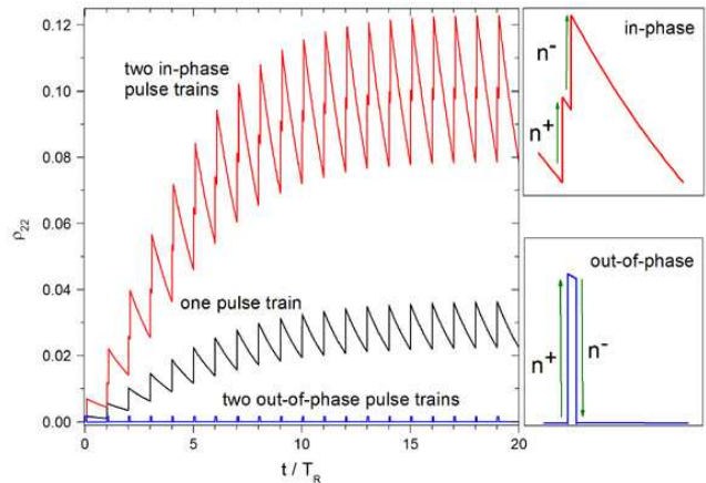
FIG. 2. (Color online) Time evolution of the excited state population ( \rho_{22} ) of ^{87}\text{Rb} -like atoms excited by a single pulse train [black curve; configuration (i)], two in-phase [red curve; configuration (ii)] and two out-of-phase [blue curve; configuration (iii)] counterpropagating pulse trains delayed by \tau = 0.9 ns. Inset: zoom-in of one period ( T_R ) dynamics in the stationary state for two in-phase (red curve) and two out-of-phase (blue curve) counterpropagating pulse trains.
