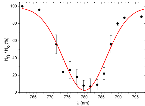
FIG. 3. (Color online) Measured trap loss as a function of the fs laser peak wavelength for the laser power of 700 mW and typical ^{87}\text{Rb} MOT parameters.
