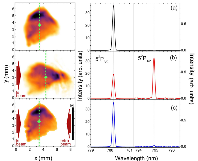
FIG. 6. (Color online) Fluorescence intensity distribution (left panel) and LIF spectra (right panel) of the cold rubidium cloud for: (a) no fs excitation, (b) excited by a single pulse train, and (c) excited by two out-of-phase counterpropagating pulse trains created by retroreflecting the fs laser beam. Green dashed line indicates the position of the CM of the cloud. Note the different intensity scales of the 780.2 nm and 795 nm LIF signals.
