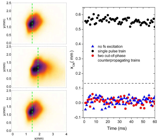
FIG. 7. (Color online) Fluorescence intensity distribution (left panel) and time evolution of the CM coordinate (right panel) of the cold rubidium cloud for the cases of no fs excitation (blue triangles), excitation by a single pulse train (black dots), and excitation by two out-of-phase counterpropagating pulse trains (red dots) created by retroreflecting the fs laser beam. Green dashed line on the left panel indicates the position of the CM of the cloud. Black dashed line on the right panel indicates the expected position of the cloud calculated by using Eq. (2)
