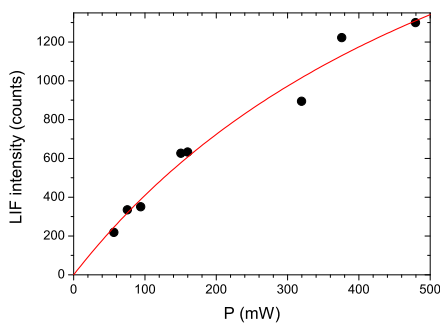
FIG. 4. (Color online) Fluorescence from the cold rubidium cloud induced by the 5S_{1/2}(F_g = 2) \rightarrow 5P_{1/2}(F_e = 1, 2) excitation using a single frequency comb (points). Data are fitted to a saturation curve (red line).
